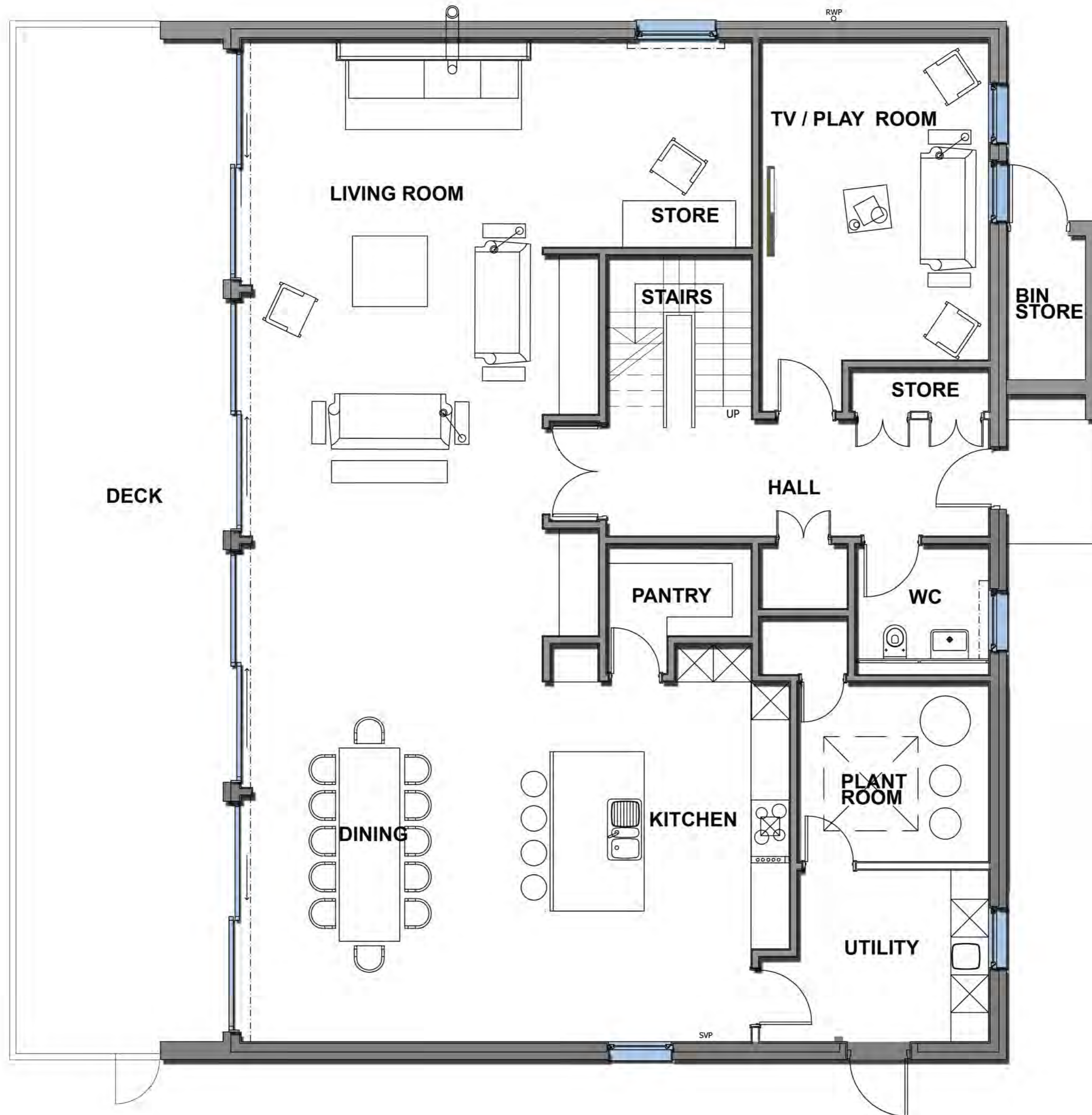
GROUND FLOOR PLAN YOO BOWMOOR
