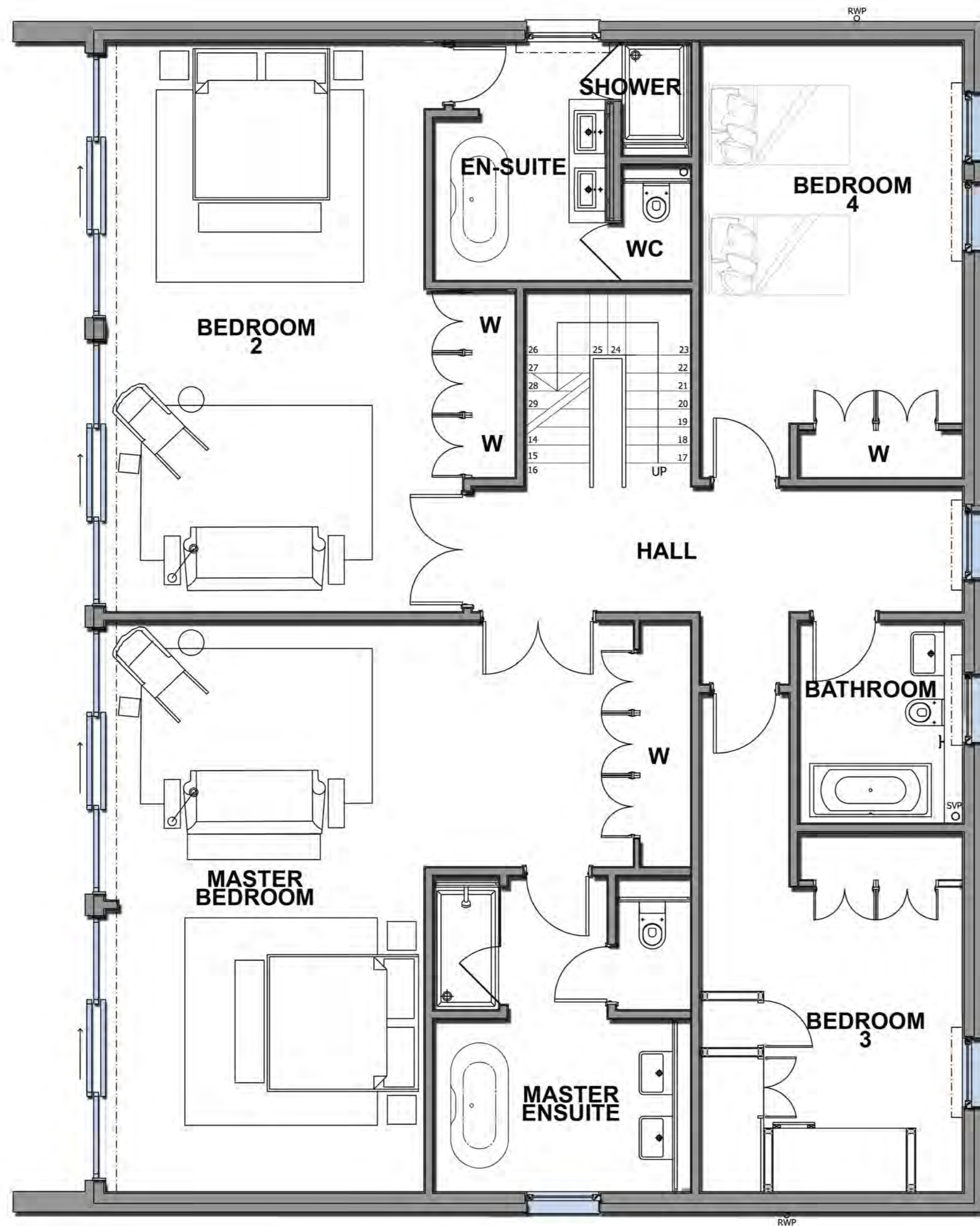
FIRST FLOOR PLAN YOO BOWMOOR
